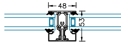
Fixed Mullion
