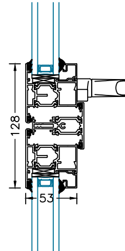
Sash Transom
